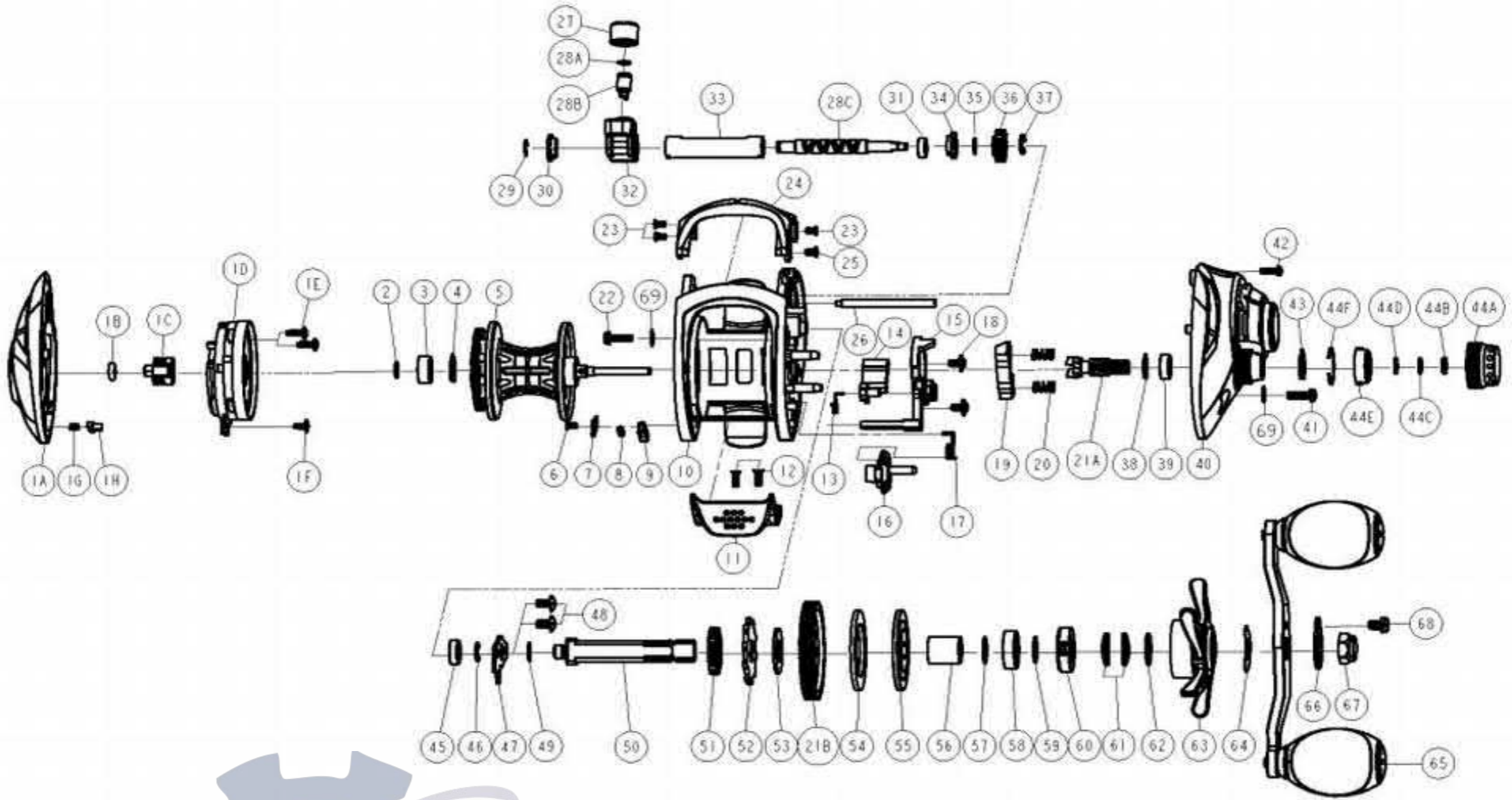
Quantum Energy T100HPTMG Baitcast Reel Part List
